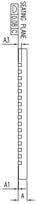
SIDE VIEW
